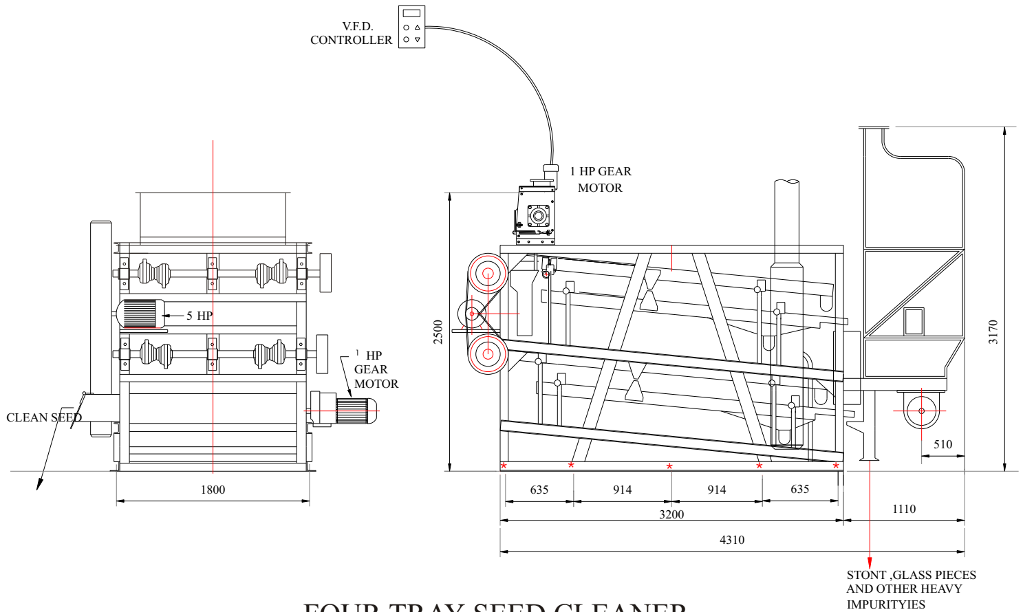
FOUR TRAY SEED CLEANER
