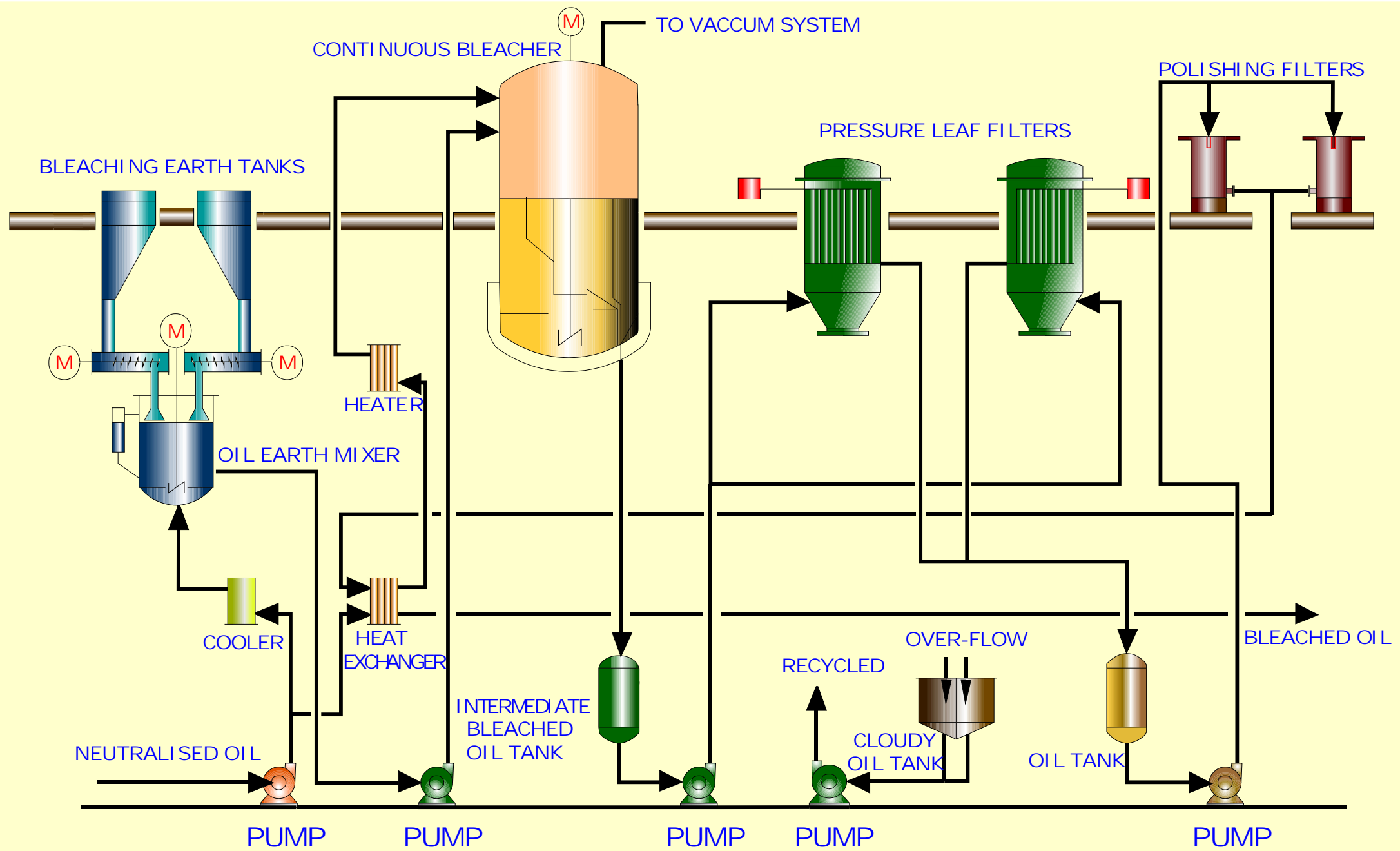
FLOW SHEET FOR CONTINUOUS BLEACHING PROCESS
