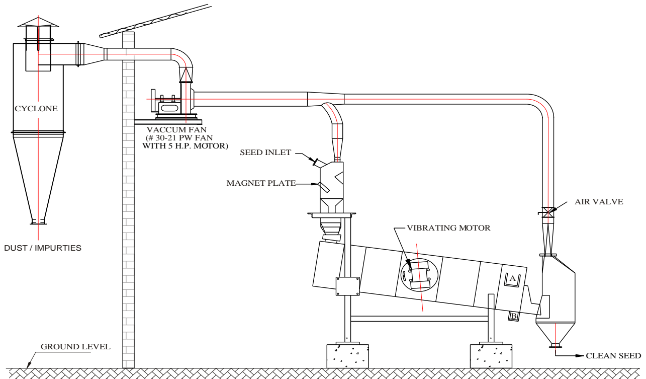
SEED CLEANER HIGH CAPACITY WITH ASPIRATION SYSTEM.
